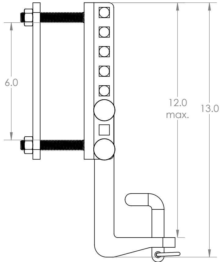
SIDE VIEW - LOWEST POSITION
