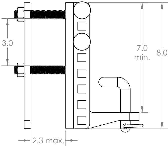
SIDE VIEW - HIGHEST POSITION
