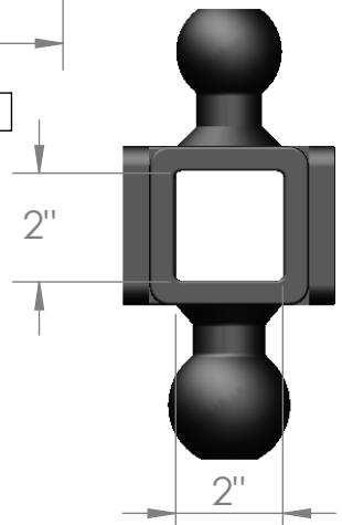
SLIDER VIEW
